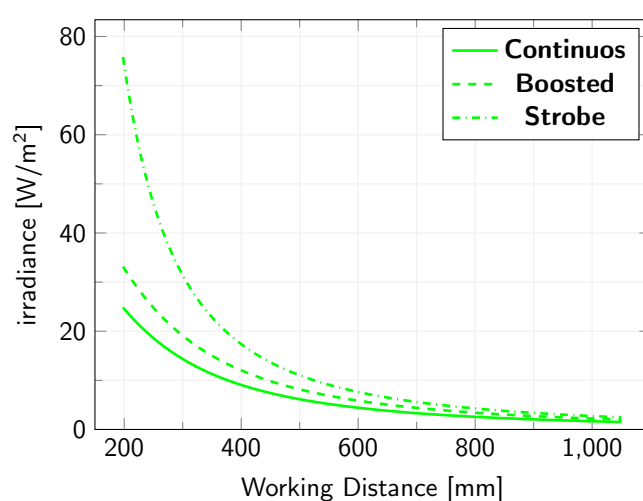
Irradiance Characteristics
